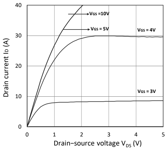
Figure 1. Output Characteristics
