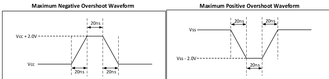
Figure-77. Maximum Negative/positive Overshoot Diagram
