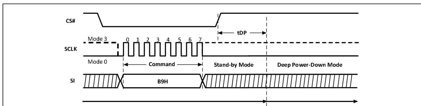
Figure-51. Deep Power-Down Sequence Diagram
