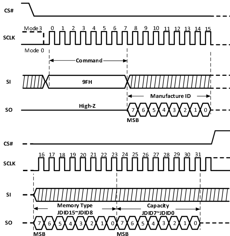
Figure-61. Read Identification Sequence Diagram
