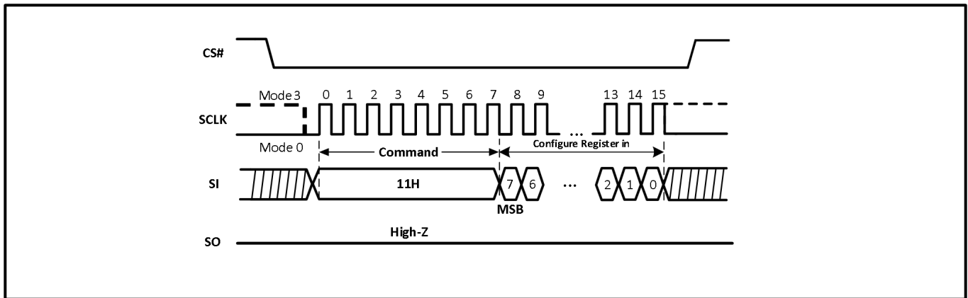
Figure-47. Write Configure Register (WRCR) Sequence (Command 11H)
