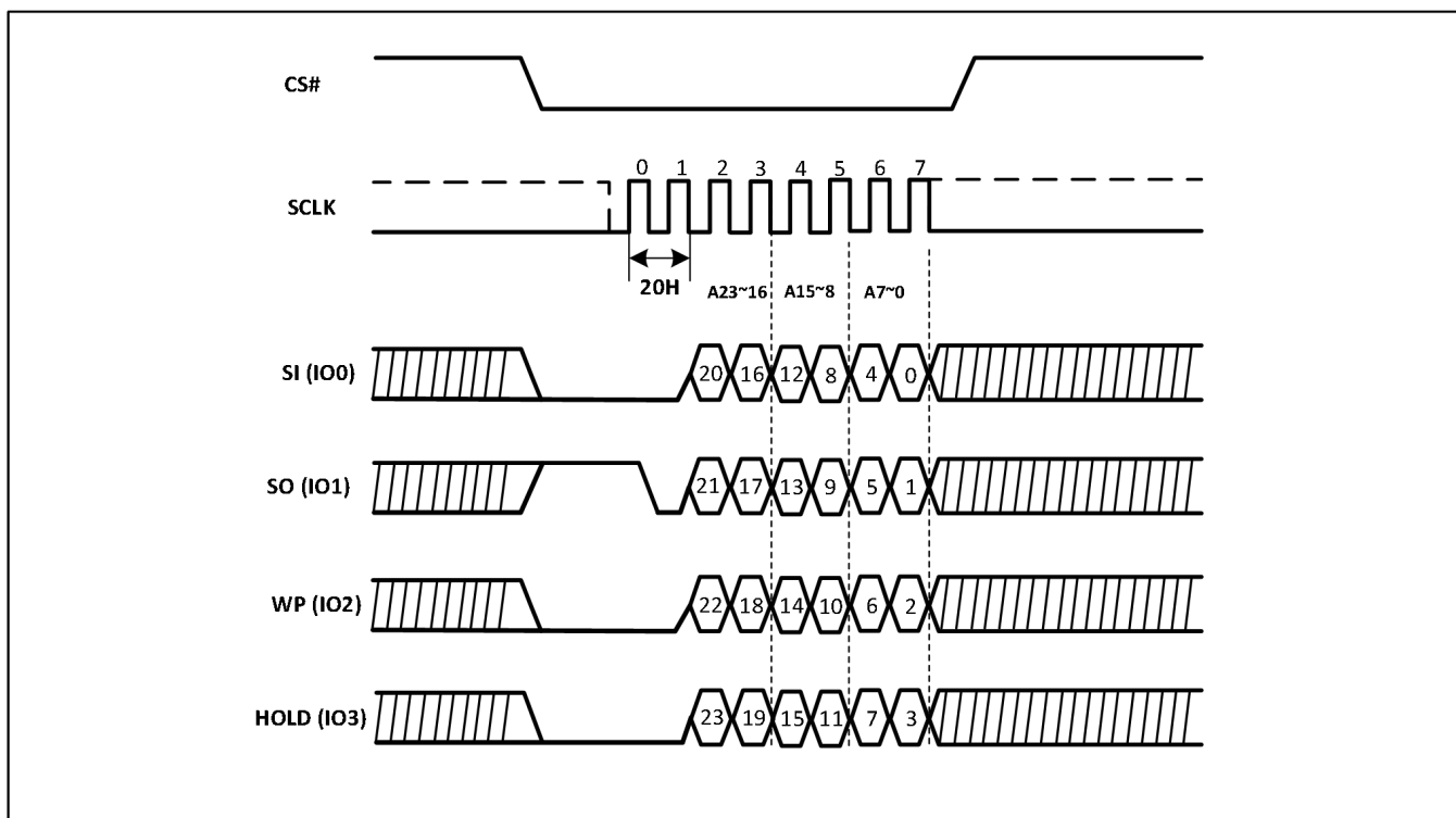
Figure-30. Sector Erase Sequence Diagram (QPI)
