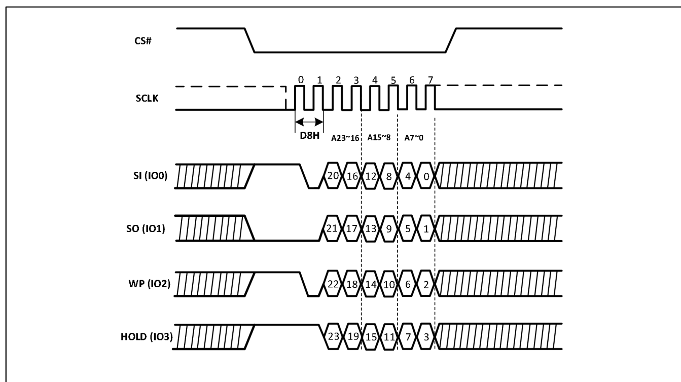
Figure-34. Block Erase Sequence Diagram (QPI)
