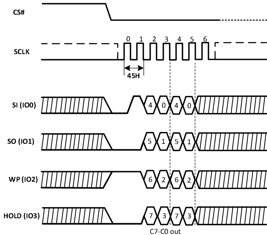
Figure-50. Read Configure Register (QPI)
