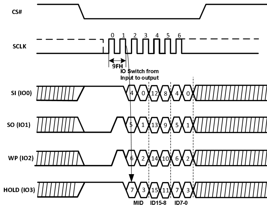
Figure-62. Read Identification Sequence Diagram (QPI)
