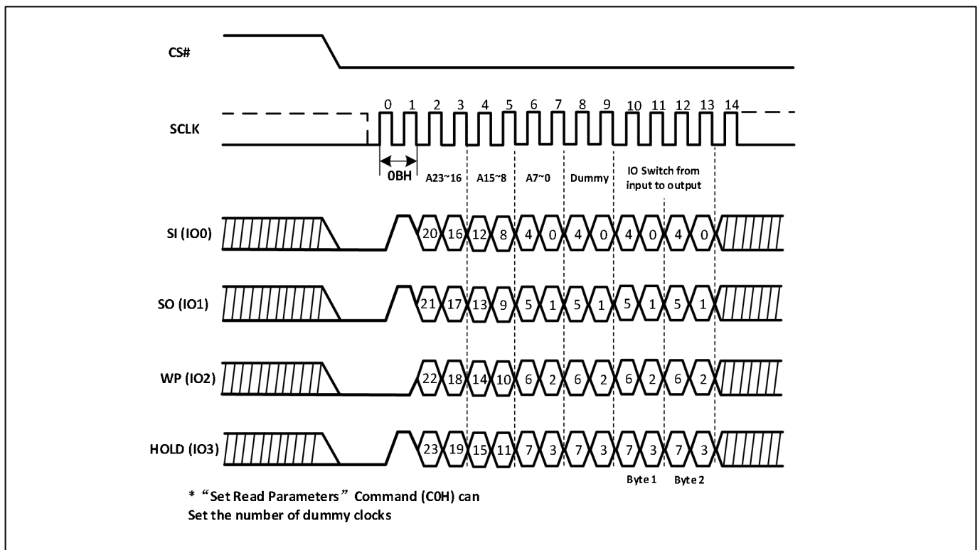
Figure-16. Read Data Bytes at Higher Speed Sequence Diagram (QPI)
