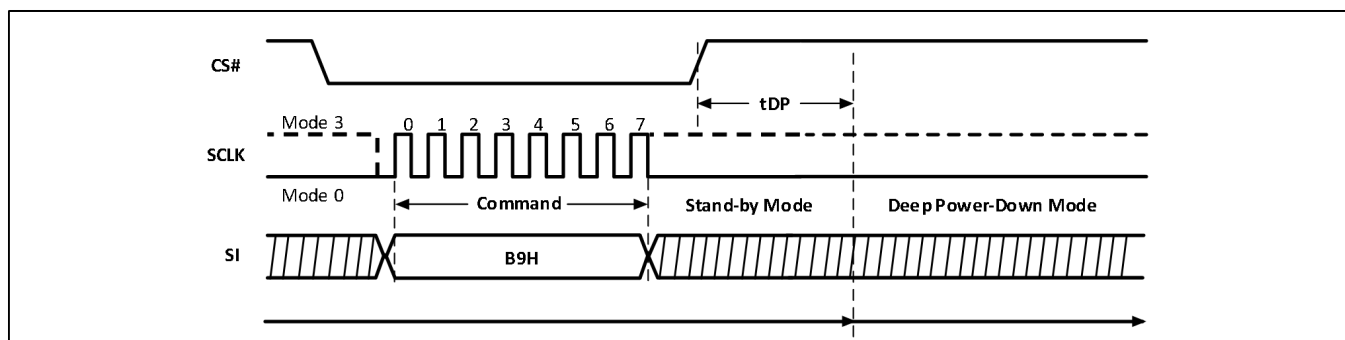
Figure-29. Deep Power-Down Sequence Diagram
